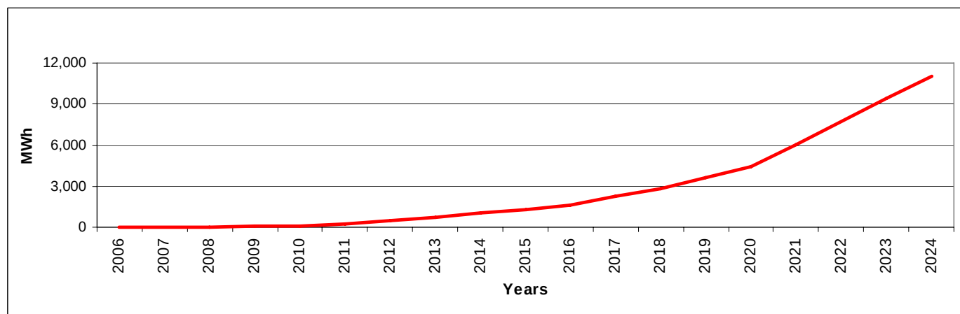
Figure 3-1-3-5A: Annual Energy Shortfall, Normal Operating Conditions
